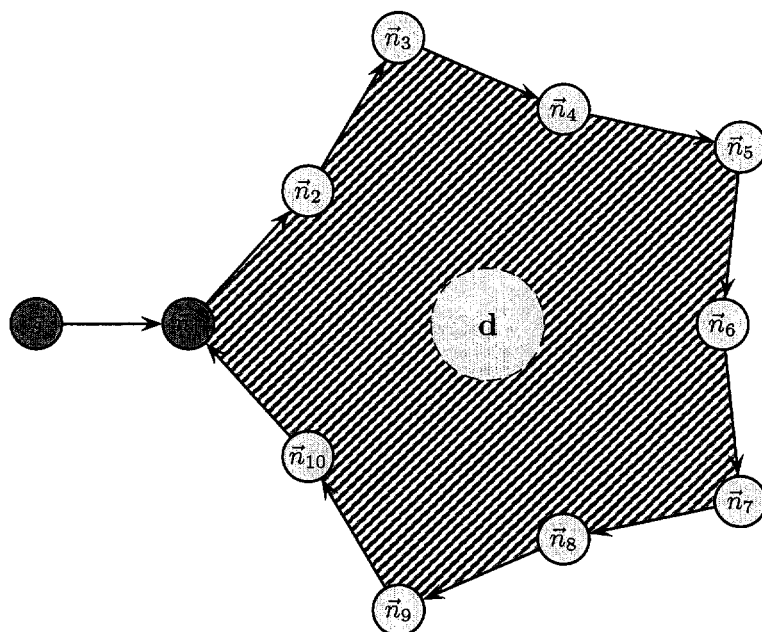
(a) A network with a wide wall around the destination.
