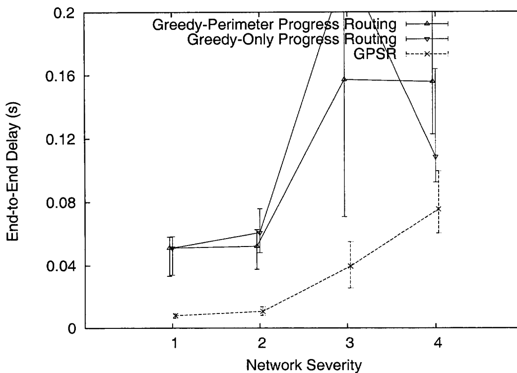
Figure 7.13. End-to-end delays with varying severity..
