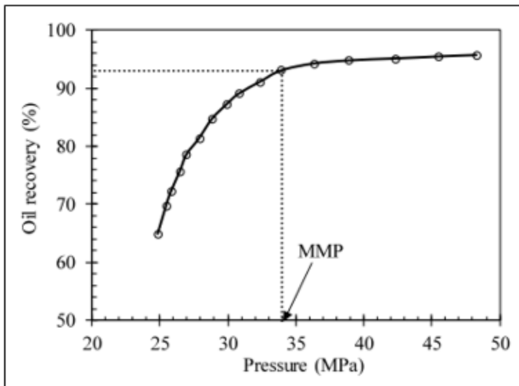
Figure 3.3.3 Representation to demonstrate when MMP reaches a steady state
