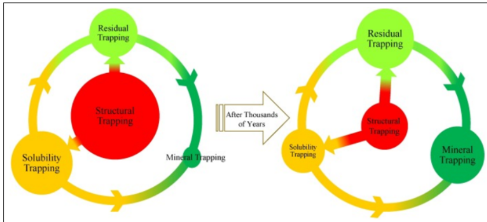
Figure 3.1.4 Change over time in structural trapping where structurally trapped CO 2 becomes more trapped residually and by solubility (Hosseini-noosheri, et al., 2018).
