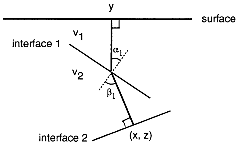
FIG. 4.2. Two-layer model.
