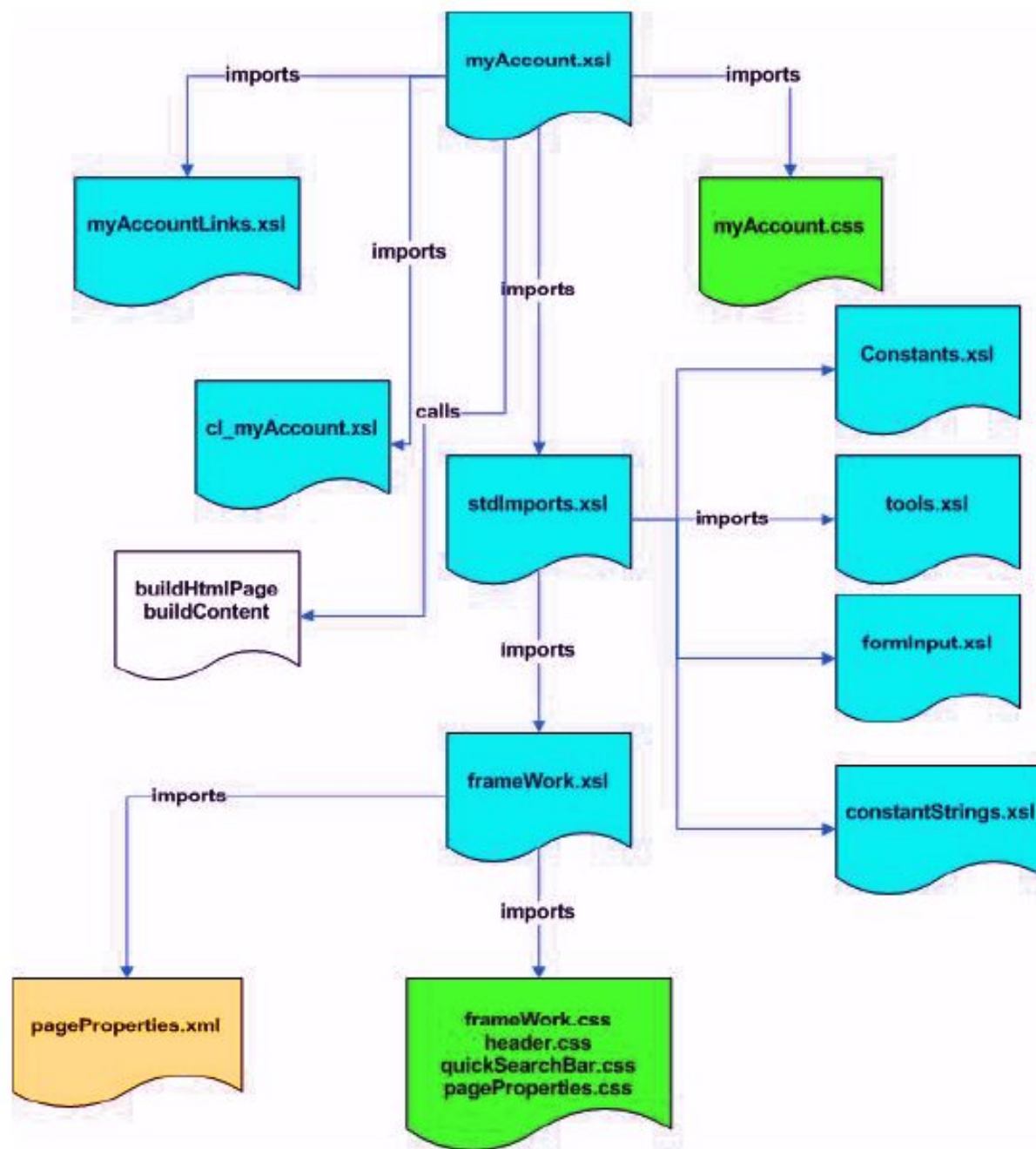
Figure 2-2. Flowchart example for myAccount page
