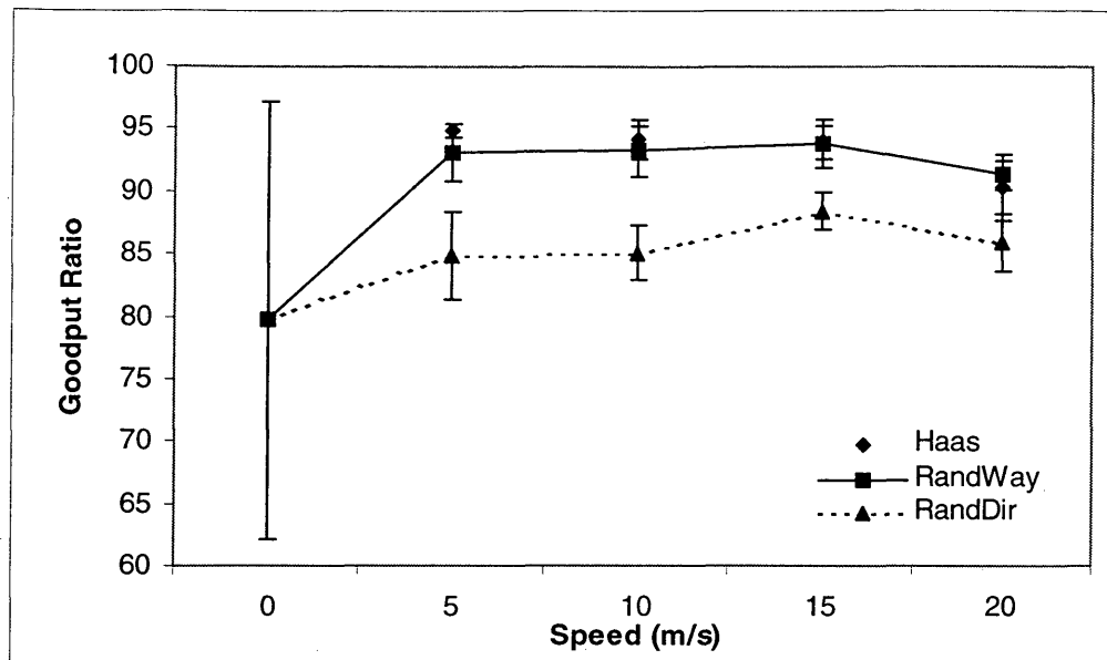
Figure 5.5 – Measure of reliability
