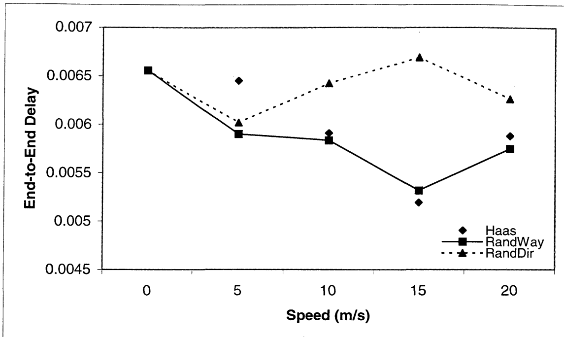
Figure 5.4 - Transmission delay
