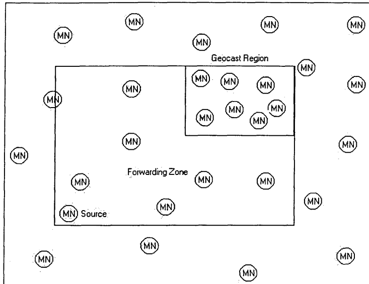
Figure 4.1 – Example simulation area using the Box approach
