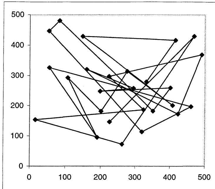
Figure 2.3 - Traveling pattern of an MN using the Random Waypoint Mobility Model
