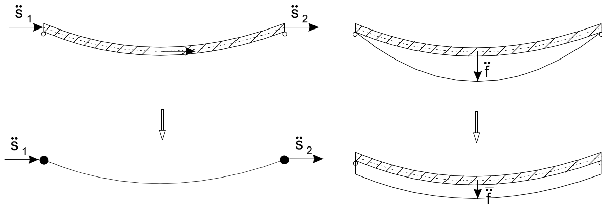
Fig. 3: Modeling of the longitudinal and vertical transversal motions of a rope span
