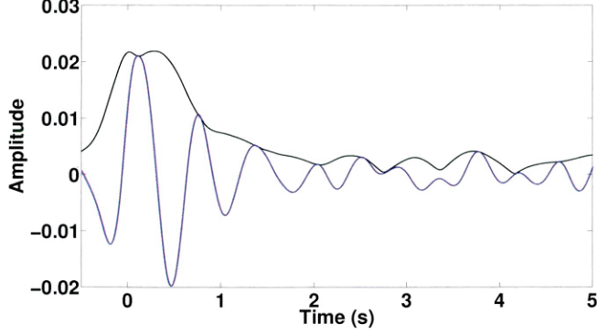
Figure 3.5: Signal from floor 4 deconvolved with upgoing waves after low band-pass filtering (blue curve). Envelope of the corresponding signal (black curve).
