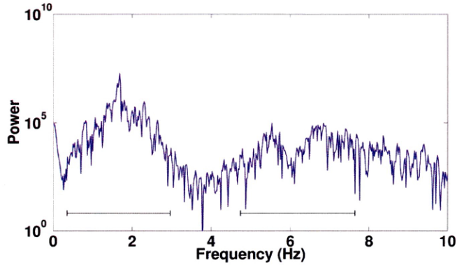
Figure 3.4: The rms power spectra of floor 7 with horizontal bars indicating the frequency bands used for band-pass filtering.
